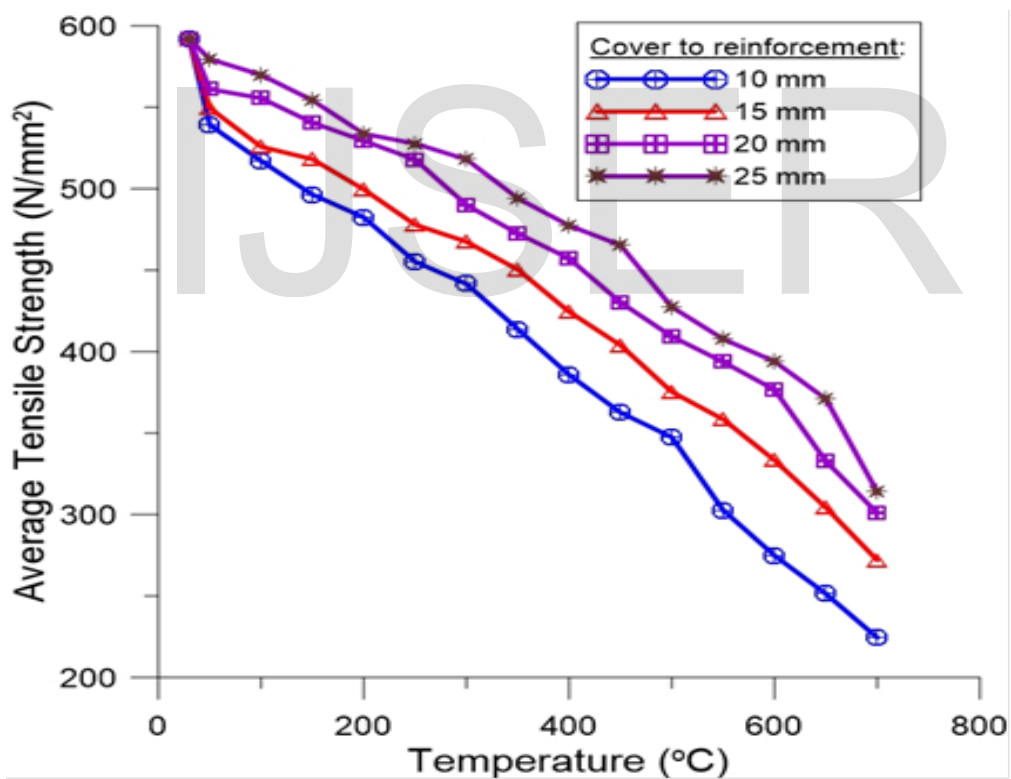
Fig. 2: Variation of average tensile strength with temperature
