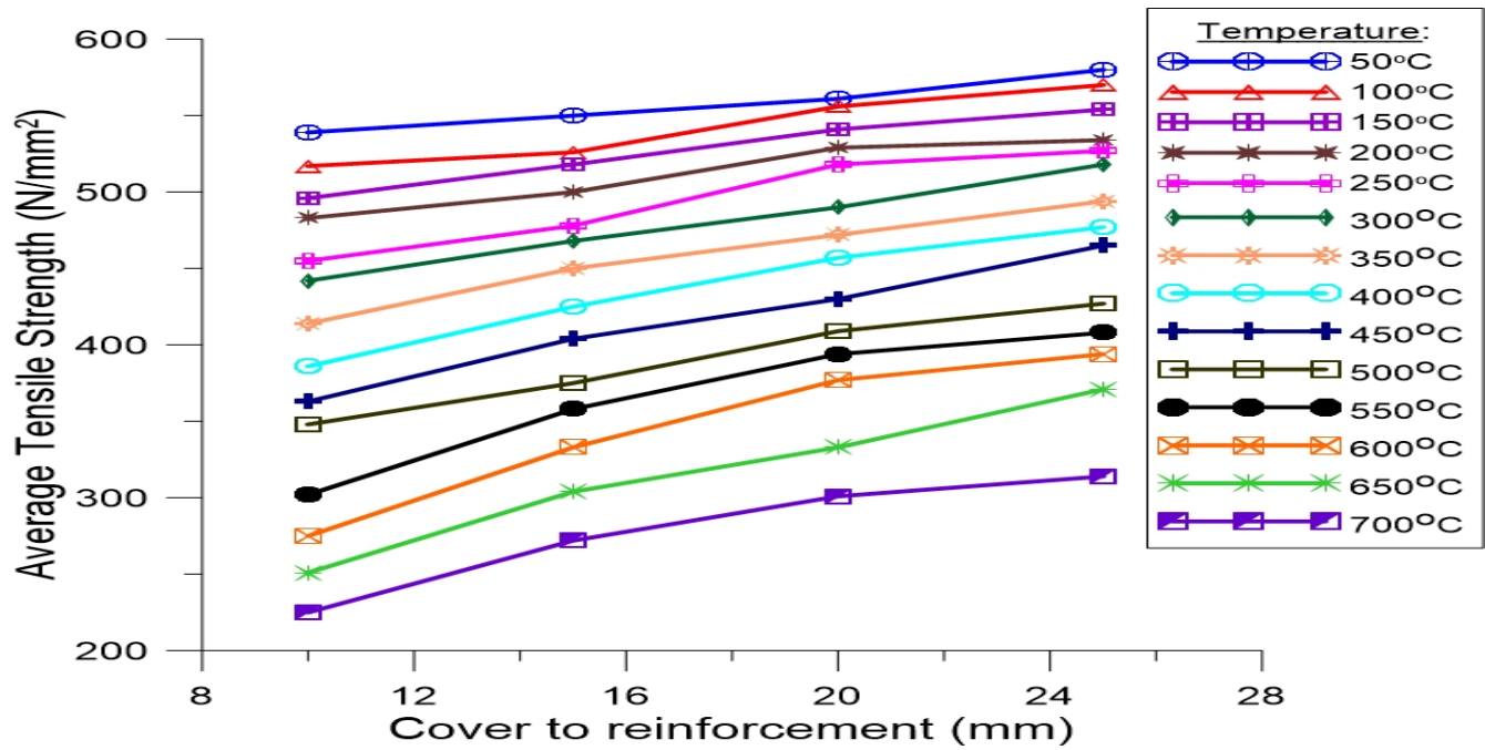
Fig.3: Variation of average tensile strength with cover to reinforcement
